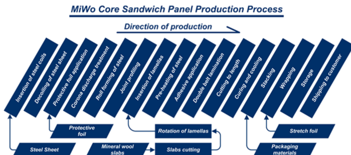
Figure 2. A scheme of WoMi sandwich panels production process by ARPANEL – sandwich panels, Adamietz Sp. z o.o
